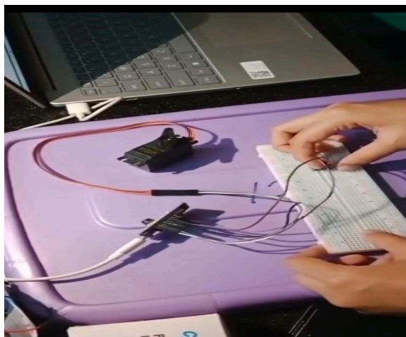
Figure 3.1.1- Circuit Setup for Task a Pushbutton for manual control of servo panning
