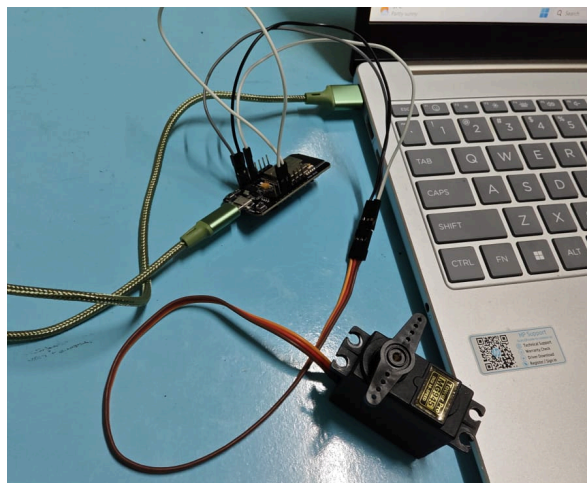
Figure 3.1.2- Circuit Setup for ESP32-CAM and Servo Motor
